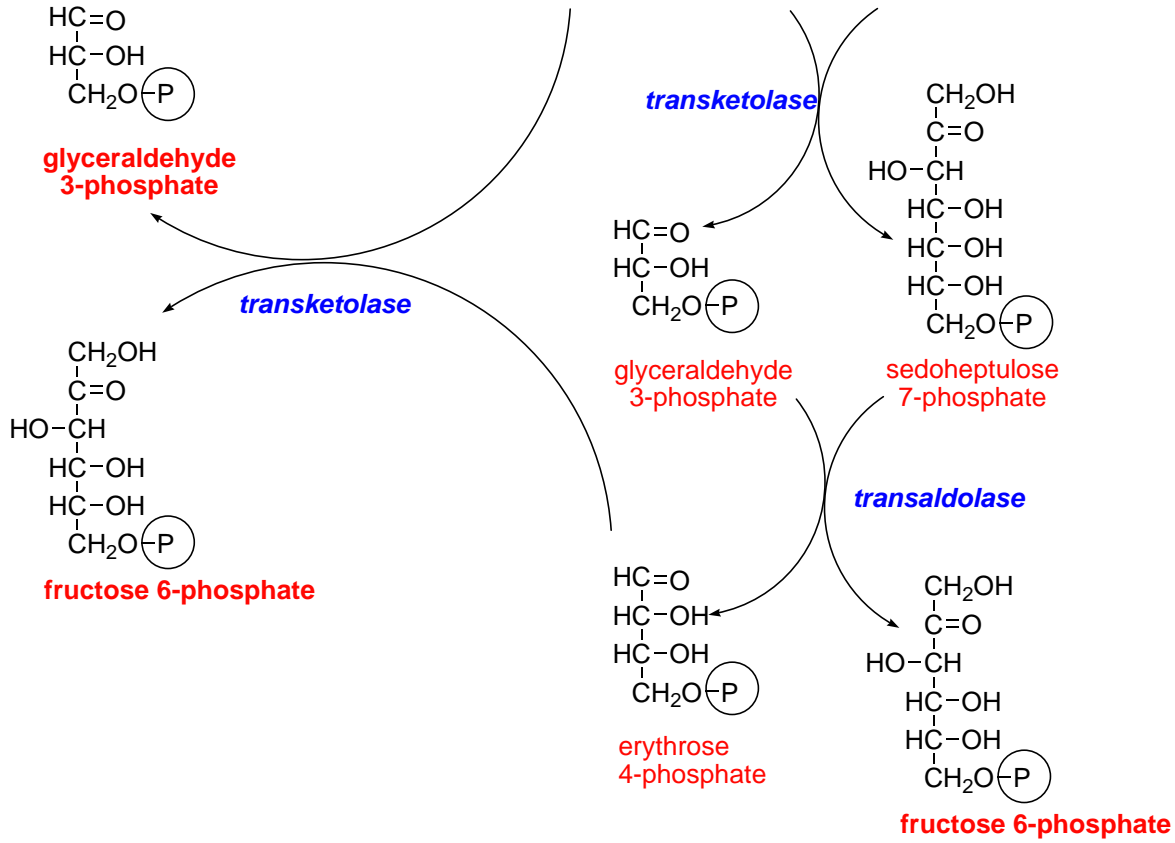
xylulose 5-phosphate ribose 5-phosphate
