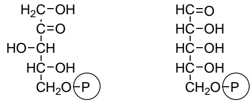
xylulose 5-phosphate ribose 5-phosphate
